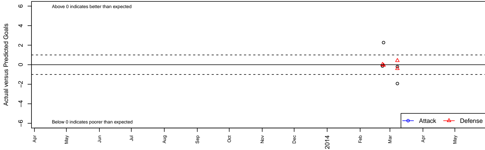
Oxnard PAL Blue B00 Dots are actual minus expected GF (blue circles) and GA (red triangles). Blue line is smoothed change in attack strength. Red is smoothed change in defense strength.
